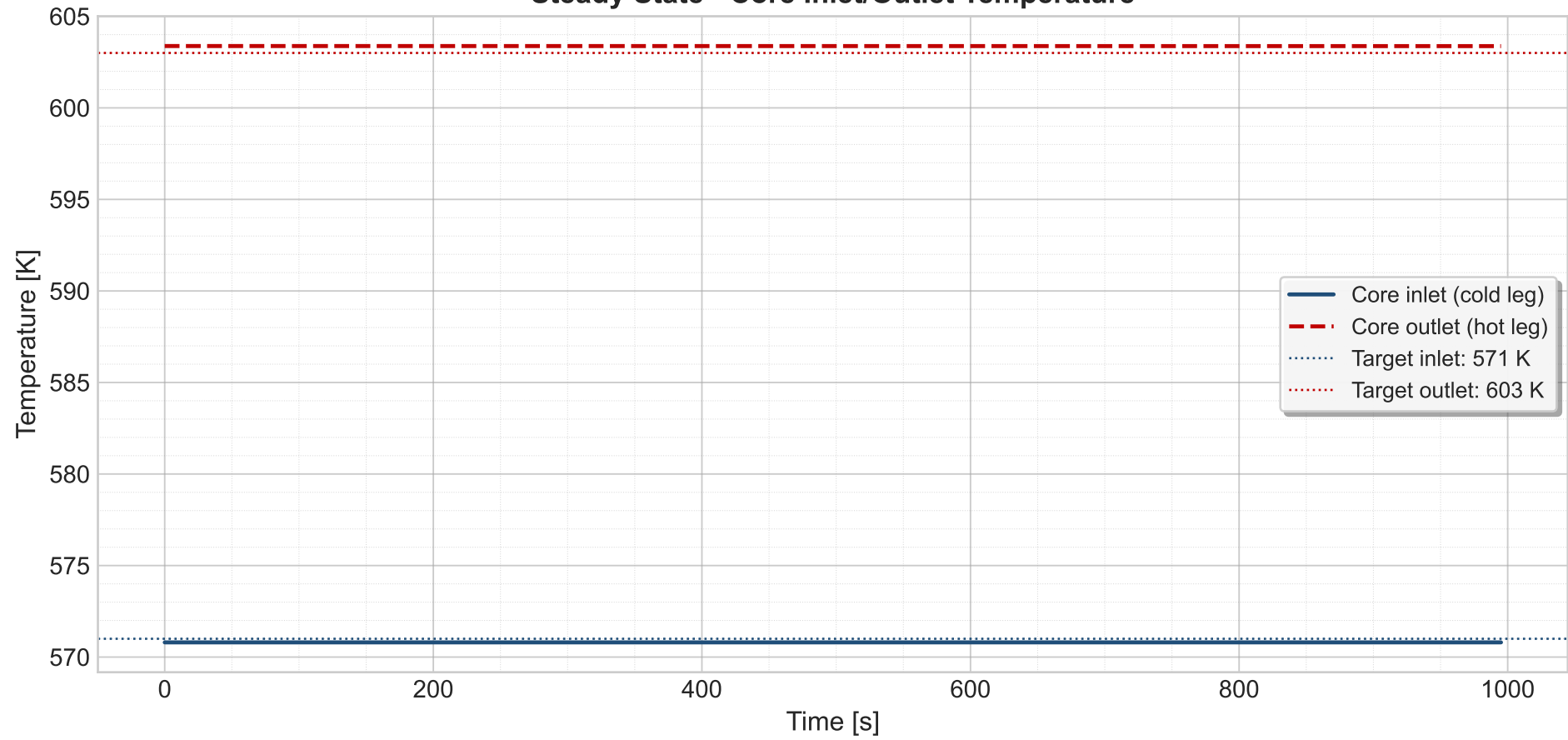
Steady State - Core Inlet/Outlet Temperature
